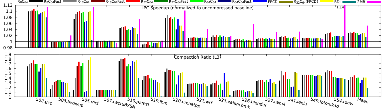
Fig. 5. Comparison of the R_YC_X compressors with the encoding stored in the data entry versus in the tags. Top plot is the IPC speedup, normalized to an uncompressed baseline. Bottom plot is the compaction ratio. Higher is better for both plots.
