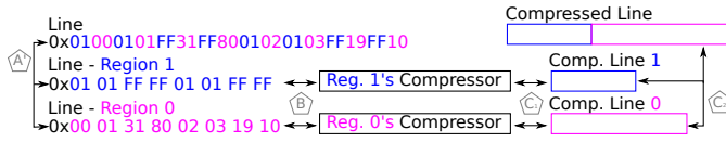
Fig. 2. A Region-Chunk compressor with two regions (MSB and LSB). Compressing and decompressing regions works by using only the regions of interest of the cache line as input to their respective compressors.
