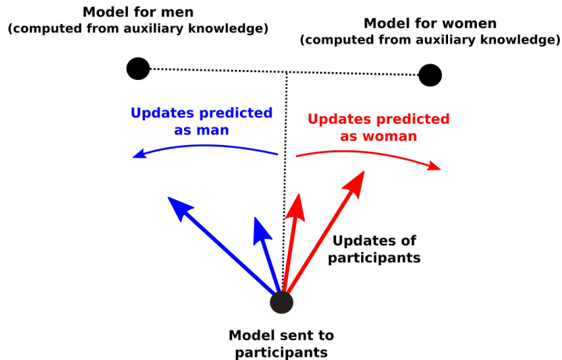
Figure 4: \nabla SIM infers attributes according to the gradient vector returned by participants (i.e., the parameter updates) and the learning models representative to each class of sensitive attributes (background knowledge).
