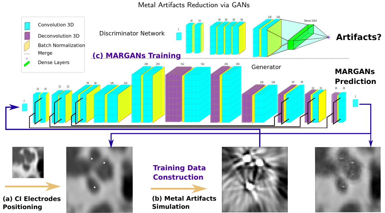
Figure 3: The framework of MARGAN for metal artifact reduction. (a) The cochlear implant positioning simulation; (b) CI metal artifact physical simulation. (c) A 3D GAN is trained with simulated and preoperative datasets. The generator outputs an image with reduced metal artifacts. The discriminator network aims to identify whether or not the input image includes metal artifacts.
