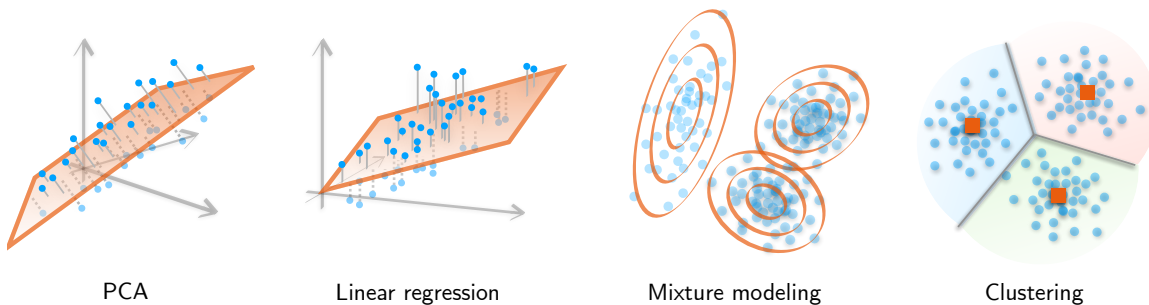
Fig. 2: Schematic representation of the four running examples covered by this paper. In the four figures, each x_i is associated with a blue colored disk, hence the training collection correspond to a point cloud, and the orange color geometrically represents the learned parameters. PCA learns the principal k -dimensional subspace of the dataset for some k \leq d . Linear regression fits observed data (the blue dot heights) as a linear model of the inputs (here, the 2-D horizontal coordinates). For least squares, this amounts to minimizing the square of the differences between these data and the linear predictions. In Gaussian mixture modeling, we learn the set of parameters (mixture weight, mean, and covariance) characterizing each Gaussian term of the mixture, which probability level sets are displayed here as orange ellipses. Clustering methods (such as k -means) learn a set of centroids (the orange squares) defining a Voronoi partition grouping together similar data samples.
