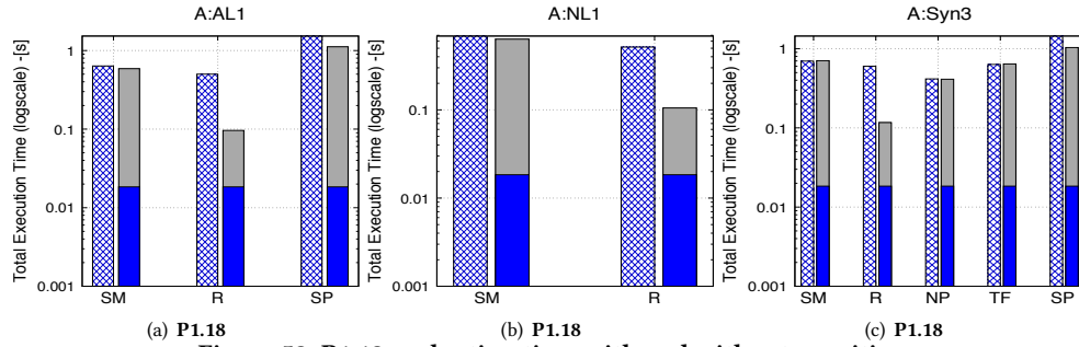
Figure 58: P1.18 evaluation time with and without rewriting
