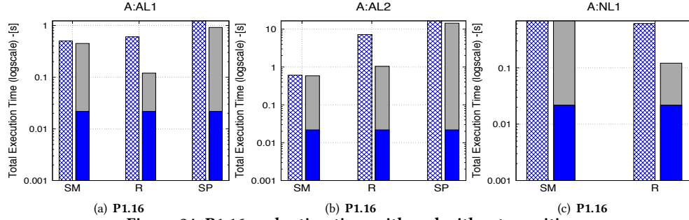
Figure 24: P1.16 evaluation time with and without rewriting
