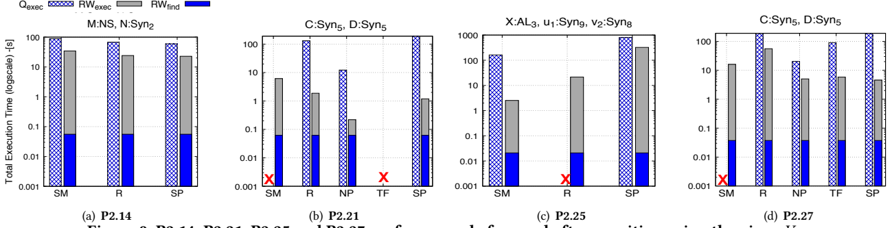
Figure 9: P2.14, P2.21, P2.25 and P2.27 performance before and after rewriting using the views V_{exp}
