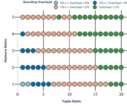
(a) P1.16 Figure 79: RW_{find} overhead as a percentage (%) of the total time ( Q_{exec} + RW_{fond} ) for pipelines 1.16 and 1.18
