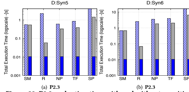
Figure 32: P2.3 evaluation time with and without rewriting
