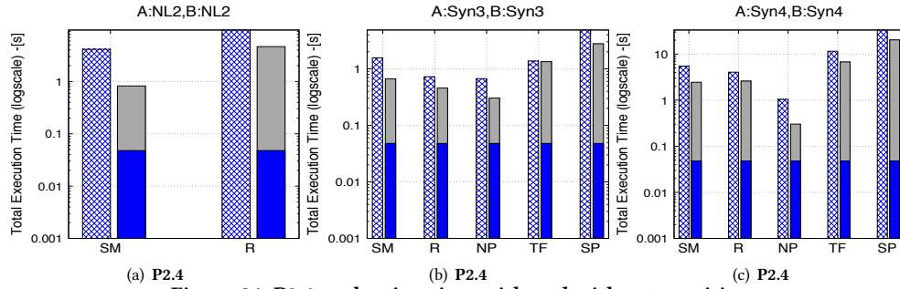
Figure 34: P2.4 evaluation time with and without rewriting
