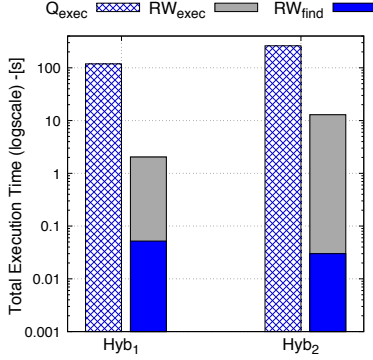
Figure 10: Hyb_1 and Hyb_2 evaluation before and after rewrite
