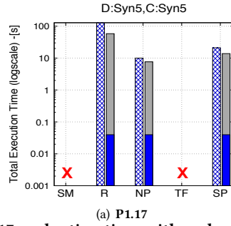
Figure 57: P1.17 evaluation time with and without rewriting
