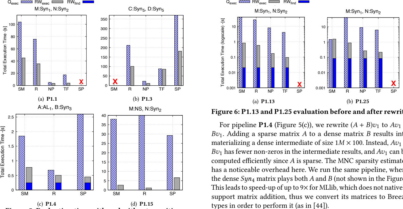
Figure 5: Evaluation time with and without rewriting
