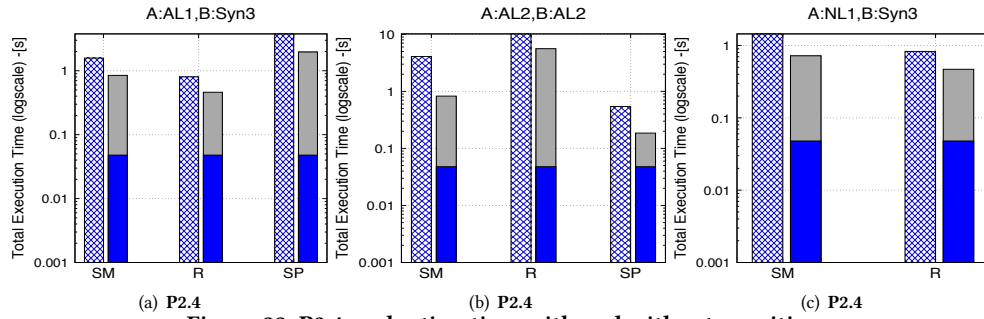
Figure 33: P2.4 evaluation time with and without rewriting
