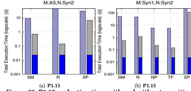
Figure 23: P1.15 evaluation time with and without rewriting
