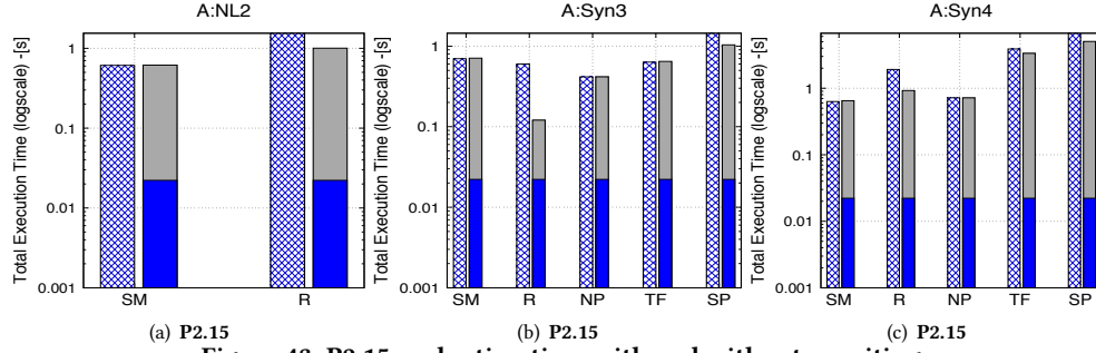
Figure 43: P2.15 evaluation time with and without rewriting
