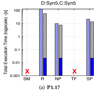
Figure 26: P1.17 evaluation time with and without rewriting
