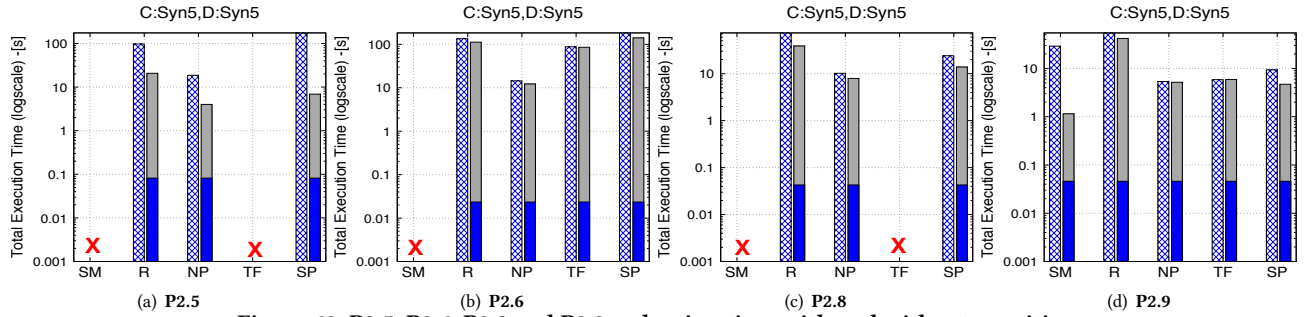
Figure 62: P2.5, P2.6, P2.8 and P2.9 evaluation time with and without rewriting
