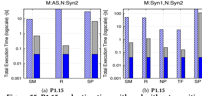
Figure 55: P1.15 evaluation time with and without rewriting
