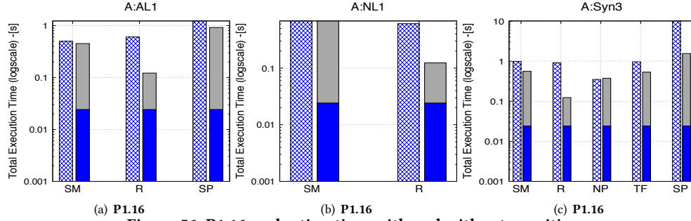
Figure 56: P1.16 evaluation time with and without rewriting
