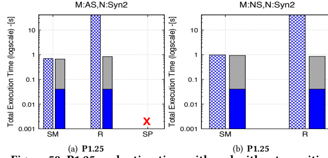
Figure 59: P1.25 evaluation time with and without rewriting
