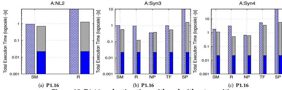
Figure 25: P1.16 evaluation time with and without rewriting
