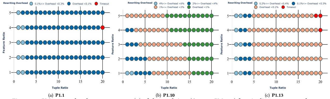
Figure 78: RW_{find} overhead as a percentage (%) of the total time ( Q_{exec} + RW_{fond} ) for pipelines 1.1, 1.10 and 1.13
