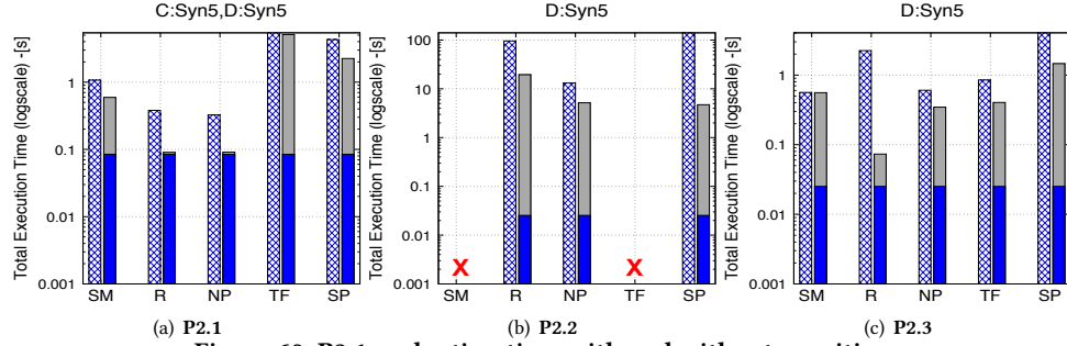
Figure 60: P2.1 evaluation time with and without rewriting
