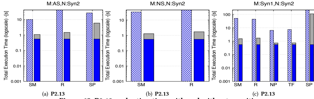
Figure 65: P2.13 evaluation time with and without rewriting
