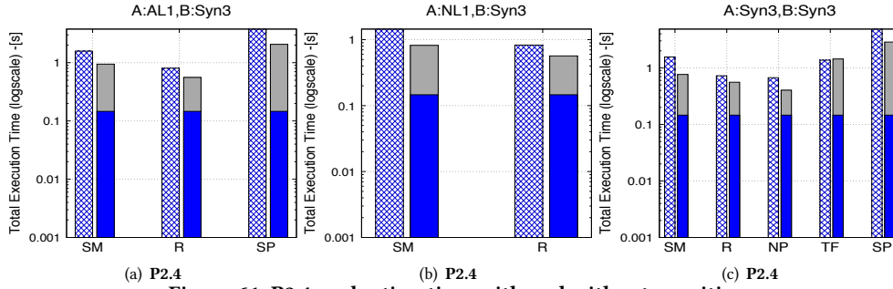
Figure 61: P2.4 evaluation time with and without rewriting
