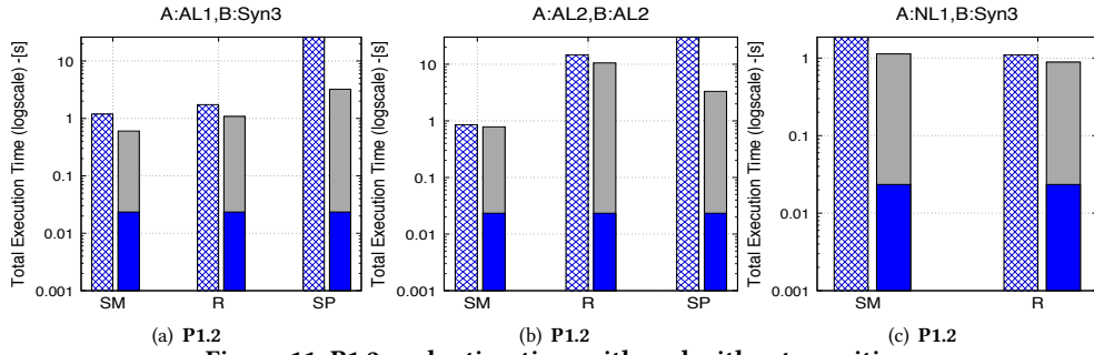
Figure 11: P1.2 evaluation time with and without rewriting
