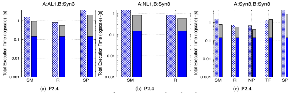
(a) P2.4 (b) P2.4 (c) P2.4 Figure 61: P2.4 evaluation time with and without rewriting
