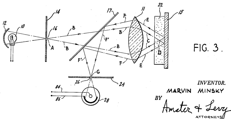
FIGURE 3.1 — Microscope confocal de Marvin Minsky (image W).
