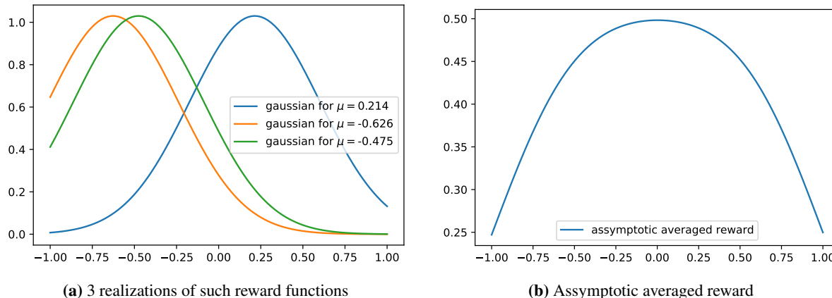
Figure 4. Gaussian adversarial reward
