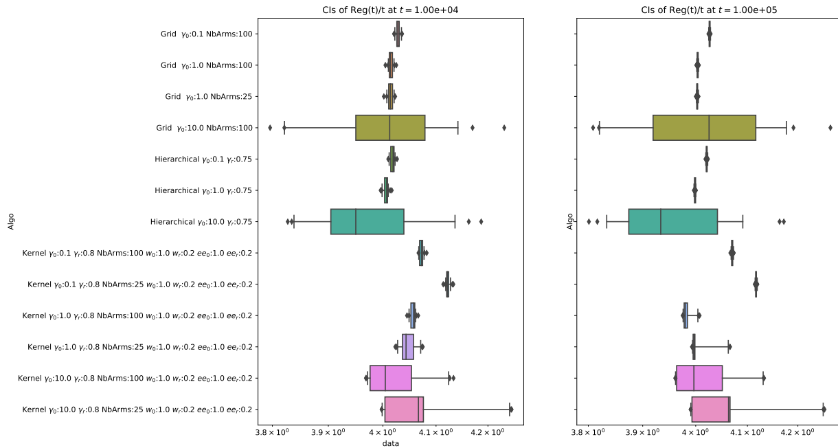
Figure 14. Distribution (moustache box are at CI of [.05, .95] ) of the averaged static regret over t , averaged on 46 realizations for each algorithm at 2 different timestamps, against the Gauss2D adversary.
