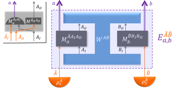
FIG. 1. SDI-QI scenario (main): A process matrix W^{AB} connects two parties who receive quantum inputs \rho_x^{\tilde{A}} and \rho_y^{\tilde{B}} , resp. They each perform a joint operation (a quantum instrument) on their quantum input and the system they receive from the process matrix ( (M_a^{\tilde{A}A_I A_O})_a and (M_b^{\tilde{B}B_I B_O})_b , resp.), and produce the classical outcomes a and b . The purple box shows the D-POVM (E_{a,b}^{\tilde{A}\tilde{B}})_{a,b} induced by these instruments and the process matrix, which acts on the quantum inputs and produces classical outputs. Inset: In the MDCI scenario, additional structure is assumed on the quantum instruments (shown here for Alice). The quantum input is a bipartite state in \mathcal{H}^{\tilde{A}_I \tilde{A}_O} , a measurement is performed jointly on \mathcal{H}^{\tilde{A}_I \tilde{A}_I} and a channel sends \mathcal{H}^{\tilde{A}_O} to the process matrix through \mathcal{H}^{\tilde{A}_O} .
