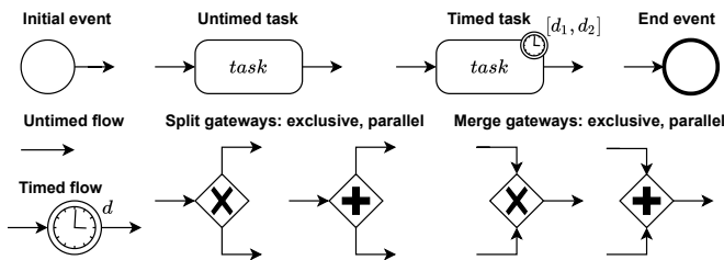
Figure 2. BPMN syntax with time features
