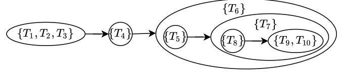
Figure 3. Initial abstract graph generated from partial order
