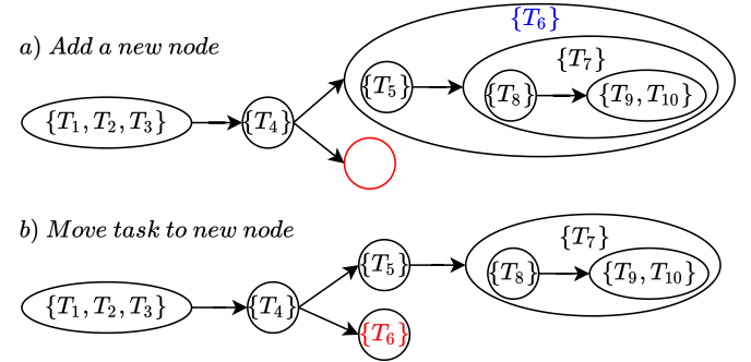
Figure 4. Example of the refinement for the running example
