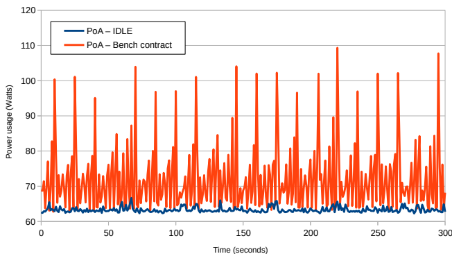
Fig. 9. Comparison power usage with and without contract execution on Ethereum PoS
