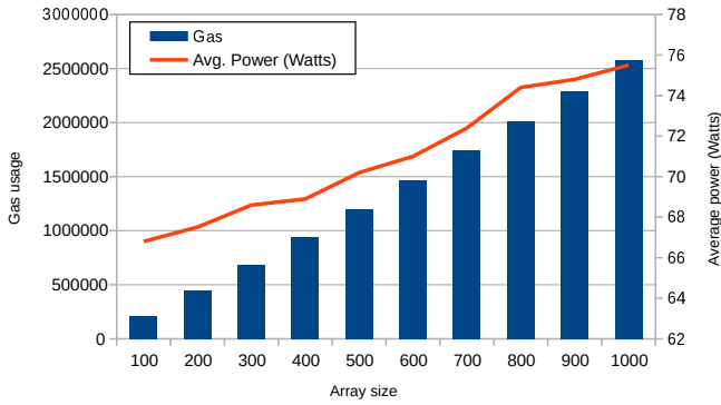
Fig. 10. Quicksort - Gas consumption and average power depending on array size input
