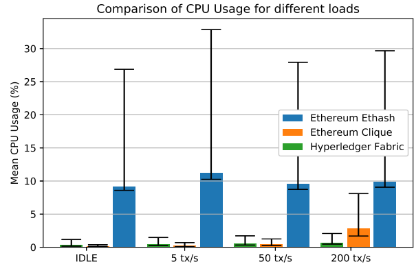
Fig. 5. Comparison of CPU Usage for different loads
