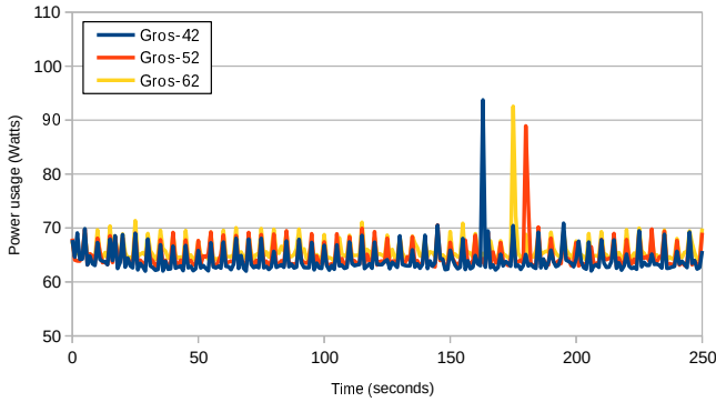
Fig. 12. Impact of smart-contract calls replication on Ethereum network energy usage
