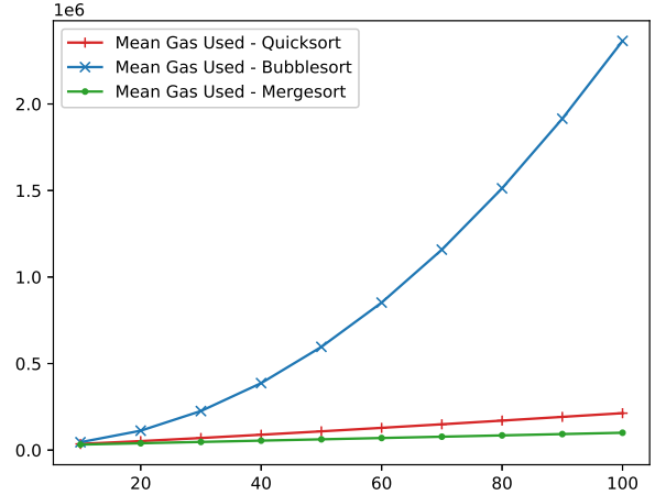
Fig. 7. Cost in gas of three smart-contracts depending on provided input
