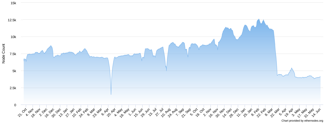
Fig. 13. Evolution of the number of Ethereum nodes listed by ethernodes.org, from October 2020 to June 2021 (source: ethernodes.org)
