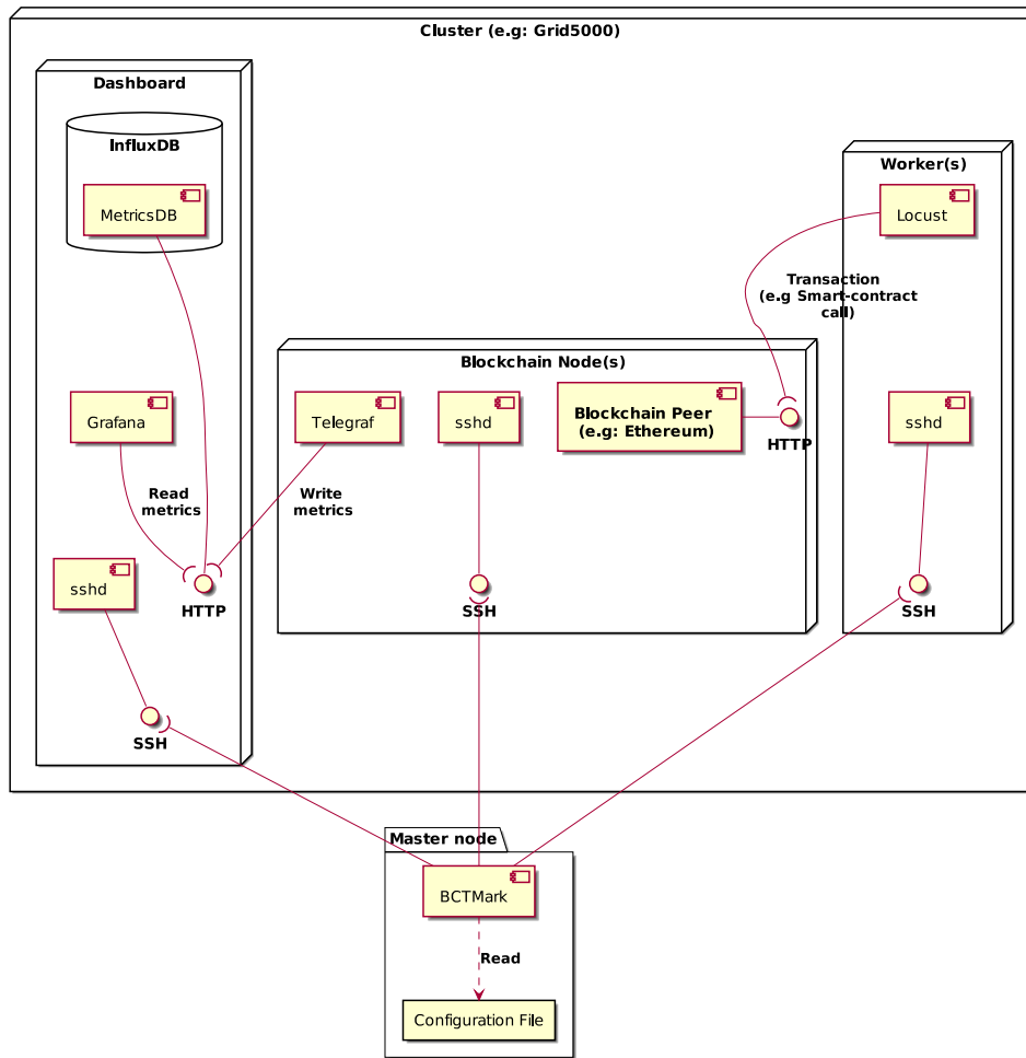
Fig. 3. BCTMark architecture
