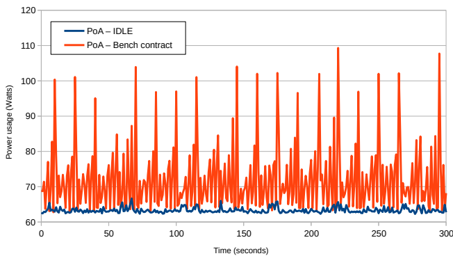
Fig. 9. Comparison power usage with and without contract execution on Ethereum PoS
