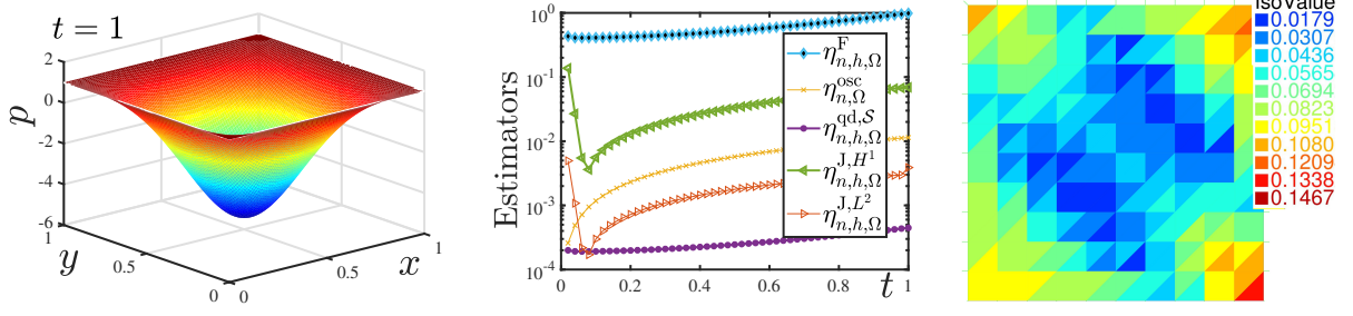
Figure 5: [Section 6.1] Exact solution p_{\text{exact}} of (6.3) at time t = 1 (left). Evolution of the 5 most significant estimators for \ell = 2 (center). The elementwise flux estimators \eta_{n,h,K}^F for \ell = 2 and t_n = 1 (right).
