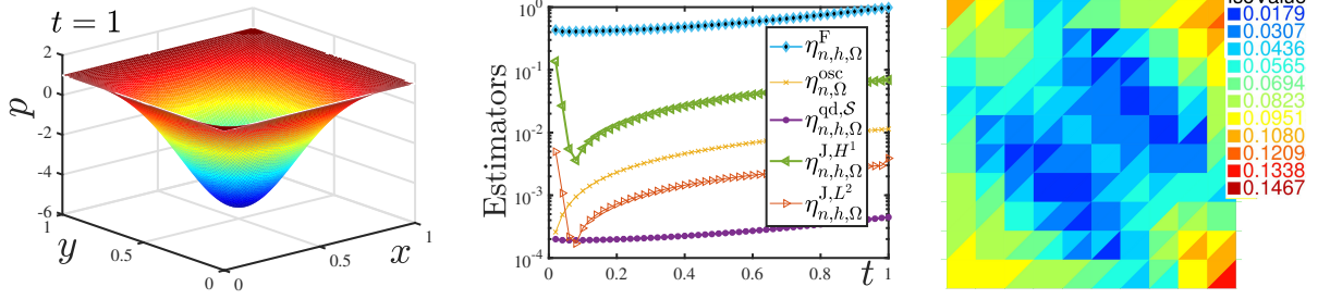
Figure 5: [Section 6.1] Exact solution p_{\text{exact}} of (6.3) at time t = 1 (left). Evolution of the 5 most significant estimators for \ell = 2 (center). The elementwise flux estimators \eta_{n,h,K}^F for \ell = 2 and t_n = 1 (right).
