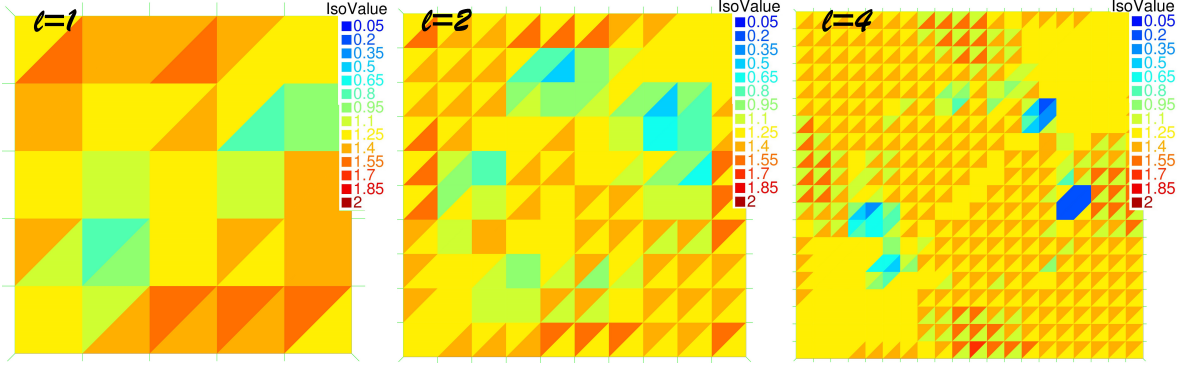
Figure 15: [Section 6.2] Local effectivity indices (6.6) for t_n = 1 and \ell = 1, 2, 4 .
