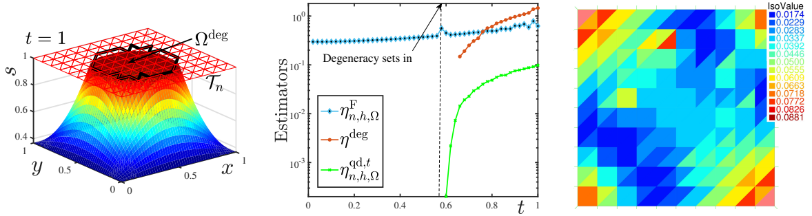
Figure 11: [Section 6.2] Saturation of the exact solution \Psi_{\text{exact}} and the domain \Omega^{\text{deg}}(t) at t = 1 (left). The principal estimators \eta_{n,h,\Omega}^{\text{F}}(t) , \eta^{\text{deg}}(t) , and \eta_{n,h,\Omega}^{\text{qd},t}(t) for \ell = 2 (center), and the elementwise estimators \eta_{n,h,K}^{\text{F}} at t_n = 1 (right).
