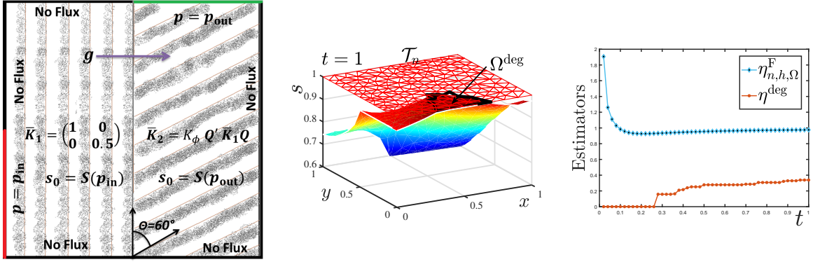
Figure 16: [Section 6.3] Computational domain showing heterogeneities, initial, and boundary conditions (left). Saturation of the numerical solution ( S_{n,h} ) for \ell = 2 at t = 1 . The mesh and the domain \Omega^{\text{deg}}(1) containing the degenerate region is shown (center). The main estimators for the same simulation (right). The flux estimator \eta_{n,h,\Omega}^F contributes the most to the error, along with the degeneracy estimator \eta^{\text{deg}}(t) which becomes non-zero only after the onset of degeneracy.
