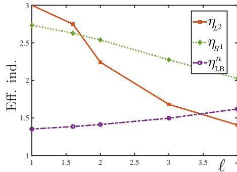
Figure 9: [Section 6.1] Effectivity indices of the estimators \eta_{L^2} , \eta_{H^1} , and \eta_{LB}^n at the final time T = 1 varying with \ell .
