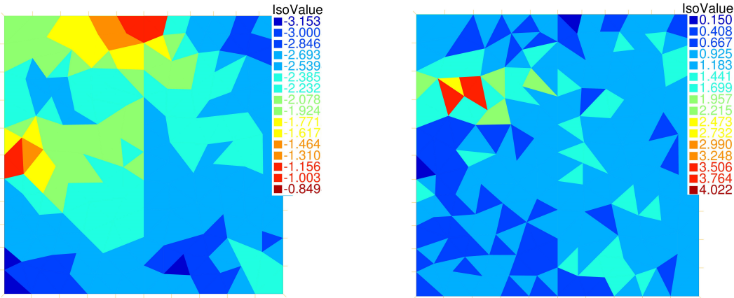
Figure 17: [Section 6.3] Elementwise distribution of \eta_{n,h,K}^F at time t = 1 in \log_{10} -scale for \ell = 2 (left). Estimators take larger values near the inlet and the outlet. Local effectivity indices defined in (6.6) (right). Here, the numerical solution for \ell = 4 is used in the place of the exact solution.
