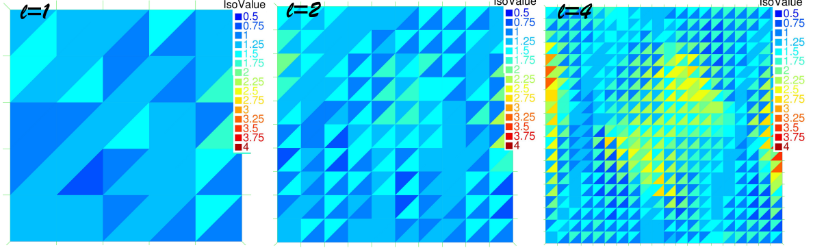
Figure 10: [Section 6.1] Local effectivity indices (6.6) at the final time T = 1 for different values of \ell .
