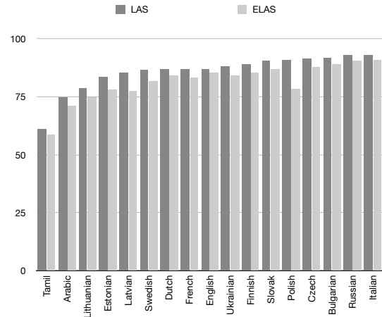
Figure 7: LAS of UDPIPE and ELAS of GREW(UDPIPE)
