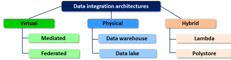
Fig. 4. The taxonomy of data integration architectures
