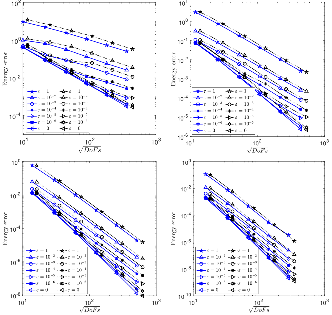
Figure 3: Polygonal domain and smooth solution. Convergence rates in the energy norm on rectangular (solid line) and polygonal (dotted line) meshes for different values of \varepsilon . The polynomial degree k = 0 (top left), k = 1 (top right), k = 2 (bottom left) and k = 3 (bottom right).
