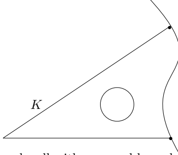
Figure 1: Example of a boundary mesh cell with a curved boundary face and which is star-shaped with respect to an interior ball; \bullet denotes a mesh vertex at the boundary.
