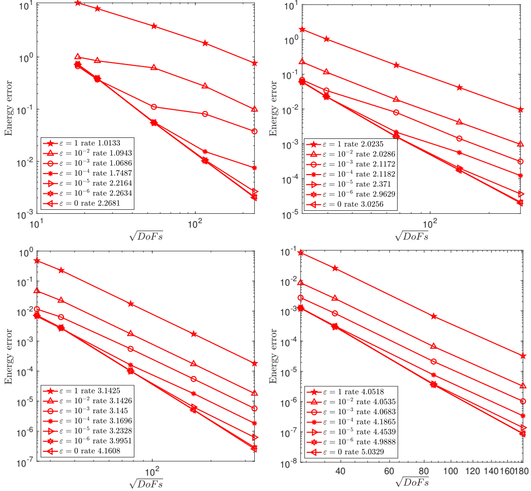
Figure 5: Annular domain and smooth solution. Convergence rates in the energy norm on curved triangular meshes for different values of \epsilon . The polynomial degree k = 0 (top left), k = 1 (top right), k = 2 (bottom left) and k = 3 (bottom right).
