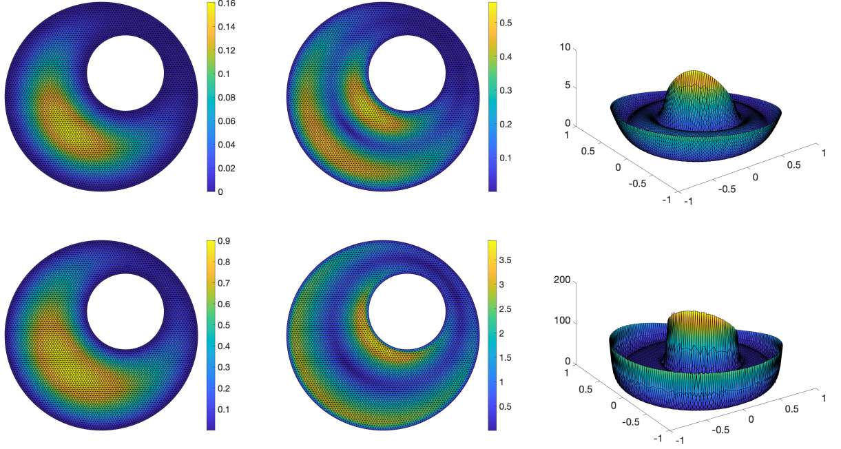
Figure 6: Test case with boundary layer on the mesh composed of 9411 cells, \varepsilon = 10^{-1} (top row) and \varepsilon = 10^{-3} (bottom row). Left column: reconstructed solution; middle column: piecewise gradient of reconstructed solution (Euclidean norm); right column: piecewise Hessian of reconstructed solution (Frobenius norm).
