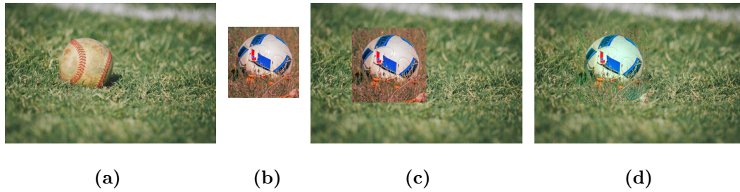
Figure 6.3: Poisson image editing. We want to replace the baseball from the image (a) with the football (b). A direct overlay leads to an unsatisfactory result (c), whereas the Poisson image editing produces an image with much less visible seams (d).
