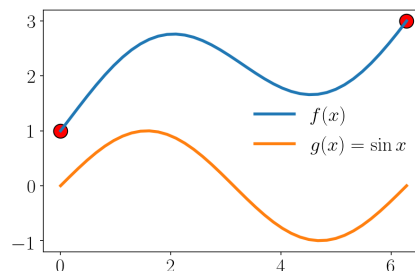
Figure 6.2: 1D Poisson's equation: the function f(x) is constrained at the extremities and it has the same second derivative as g(x) .
