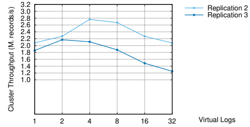
Fig. 16: Ingestion of 512 streams varying the number of virtual logs. 8 concurrent producers and consumers, 4 brokers, chunk size 1 KB.
