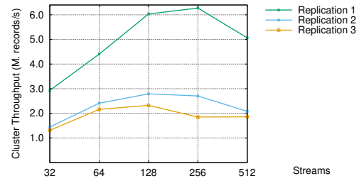
Fig. 12: Scaling the number of streams in KerA. One replicated virtual log per broker is shared for the replication of up to 512 streams. Replication 1, 2 and respectively 3 corresponds to one, two, and respectively three copies of data. 8 concurrent producers and consumers, 4 brokers, chunk size 1 KB.
