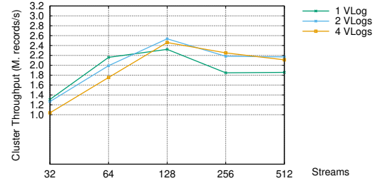
Fig. 13: Increasing the replication capacity (1, 2 and 4 shared replicated virtual logs per broker) while scaling the number of streams. Replication factor three, 8 concurrent producers and consumers, 4 brokers, chunk size 1 KB.
