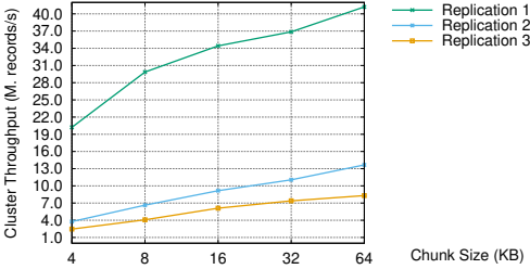
Fig. 19: One virtual log per sub-partition. The Cluster throughput corresponds to 16 producers running in parallel with 16 consumers. 4 brokers, 32 shared virtual logs per broker.
