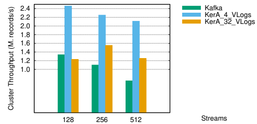
Fig. 10: Low-latency configuration. Kafka versus KerA while varying the number of streams, replication factor three with the chunk size of 1 KB. The Cluster throughput corresponds to 4 producers running in parallel with 4 consumers on 4 brokers. KerA is partitioned similarly to Kafka, one streamlet (partition) per stream with one active sub-partition per streamlet (no parallel appends). KerA has 2 configurations for stream replication, with 4 and respectively 32 virtual logs per broker.
