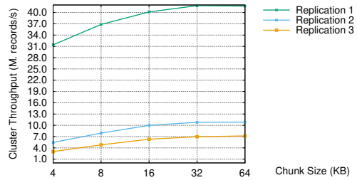
Fig. 20: One virtual log per sub-partition. The Cluster throughput corresponds to 32 producers running in parallel with 32 consumers. 4 brokers, 32 shared virtual logs per broker.
