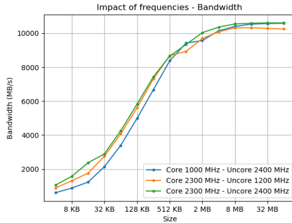
(b) Impact of constant frequencies on network bandwidth
