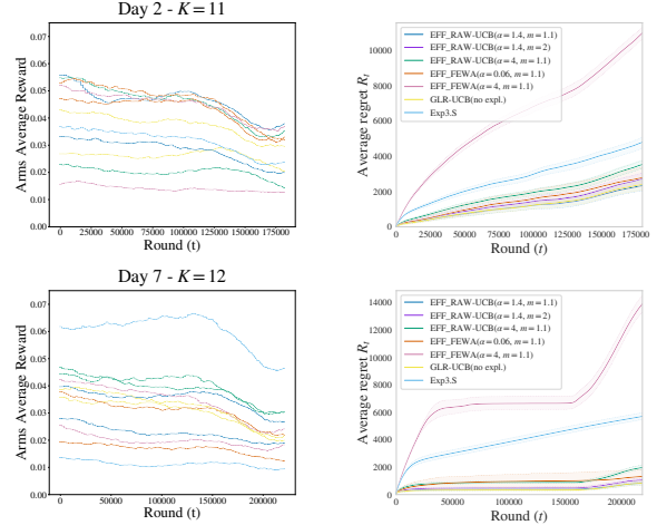
Figure 1: Left : rewards from the Yahoo! dataset for two days. Right : average regret over 500 runs.
