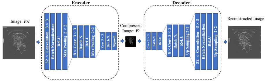
Fig. 3. The utilized AutoEncoder’s architecture
