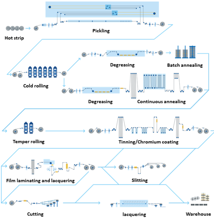
Fig. 1. Cold rolling process scheme.
