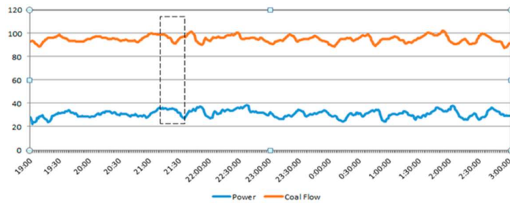
Fig. 2. Correlated power and coal flow of Coal mil. [10]
