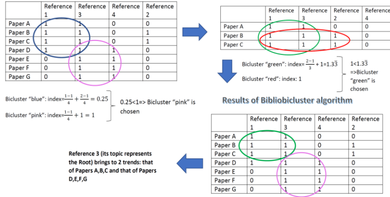
Fig. 9. BIBLIOBICLUSTER applied to the second example with \lambda = 0
