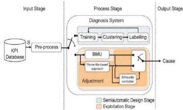
Fig. 3. Automatic root cause analysis workflow [23]
