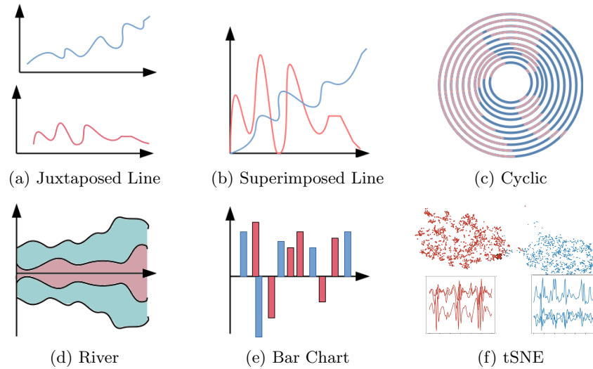
Fig. 4: A selection of plotting techniques suited to time series data. The juxtaposed and superimposed line plots are useful for comparing linear signals, as is the bar chart. The cyclic plot is best used for finding periodicities in cyclic series. River plots can be used for percentage estimation. tSNE allows full dataset exploration. (f) shows a tSNE plot of two classes of data juxtaposed with line plots of an instance from each class.
