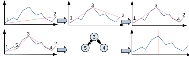
Fig. 3: A simplified demonstration of SB-Tree segmentation as outlined in [27]. PIPs are identified, built into a tree (the first and last point are generally excluded), and the roots of each tree are considered first to be a cut point for segmentation.
