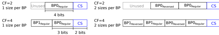
Fig. 4. A comparison of size-related metadata used at different compression factors for different configurations. CS is the compressibility state (whether CF is 1, 2, or 4). When CF=1, only the CS field is used ( i.e. , the block is not compressed).
