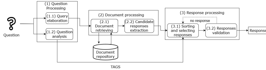
Fig. 1: Basic architecture of QA systems.
