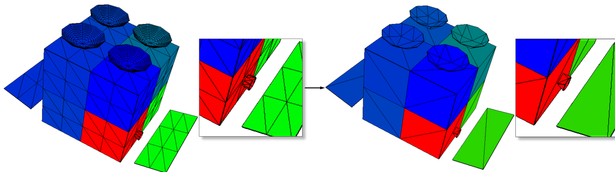
Fig. 12: Thermal simulation applied to a reduced model with prediction (from 1006 to 136 facets, i.e. a 90% reduction ratio).
