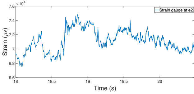
(b) Measured strain response at second sensor point
