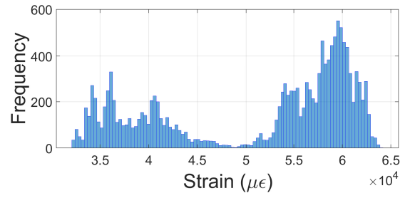
(b) Histogram of measured strain response at second sensor point
