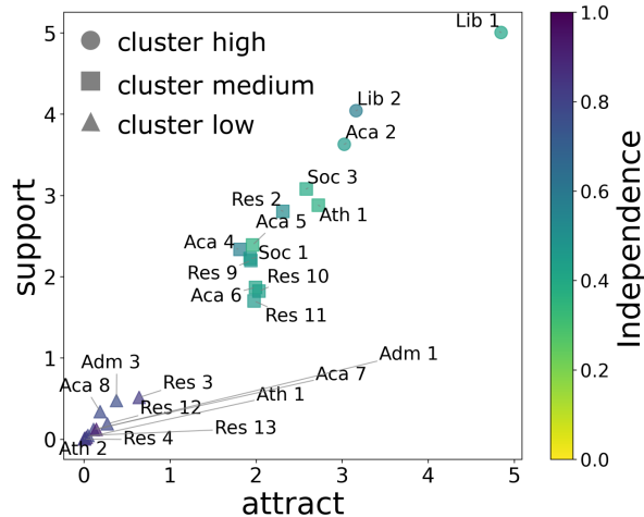
Figure 7: Relation of power among metrics
