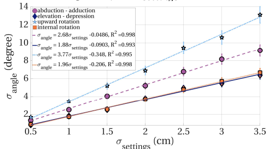
Figure 2 Relation between the std of the SL settings and the std in angle reconstruction
