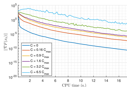
Fig. 2. rcv1: Evolution of the gradient norm along time for various noise amplitudes using S3MG algorithm.
