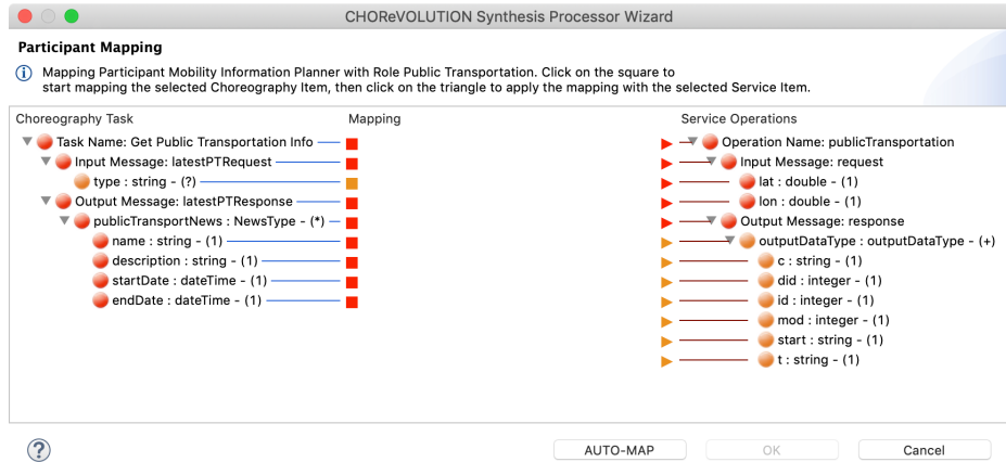
Fig. 10. Adapter Mapping
