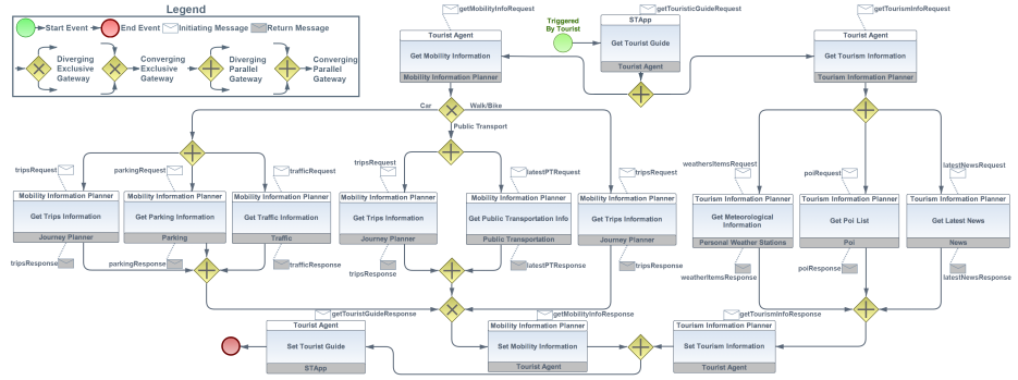
Fig. 7. Smart Mobility and Tourism choreography
