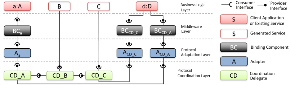
Fig. 2. Choreography architectural style (a sample instance of)
