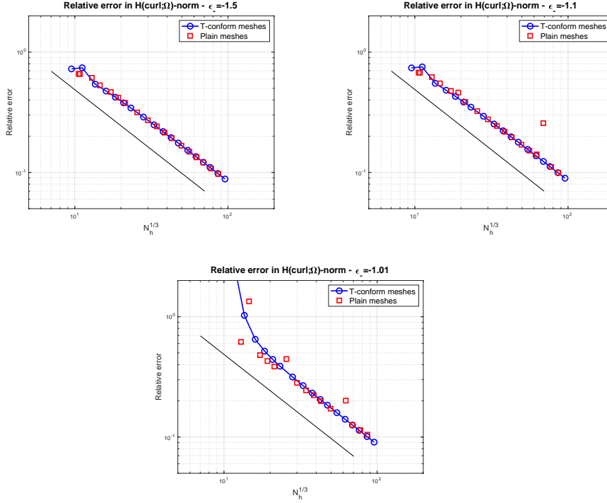
Fig. 2 Relative error in H(\text{curl};\Omega) -norm obtained for the three values of \varepsilon|_{\Omega_-} , with h varying from 0.1 to 0.01. The line corresponds to the linear scale O(h) = O(N_h^{1/3}) .
