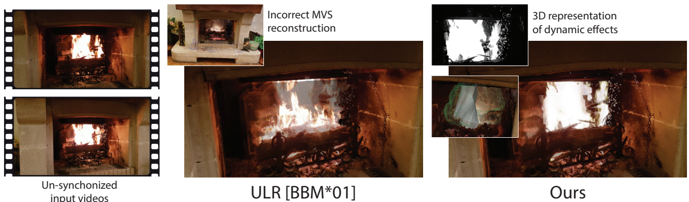
Figure 1: Unsynchronized video capture (left) is very challenging for Multi-View Stereo (MVS) and Image-Based Rendering techniques that use the resulting geometry (middle inset), where the flames have not been reconstructed. Our method enables free-viewpoint navigation in a Video-Based Rendering context for dynamic stationary effects such as fire. Our method extracts a 3D representation of dynamic effects as well as alpha-matte videos, that we use in our seamless spatio-temporal video blending scheme (left inset). When reprojecting videos onto the MVS geometry, using for example the weighting scheme of [BBM*01] (middle), the flames are incorrectly projected onto the fireplace wall. Our method (right) preserves the volumetric and semi-transparent nature of the fire during free-viewpoint rendering. These dynamic effects are best viewed in the supplemental videos.
