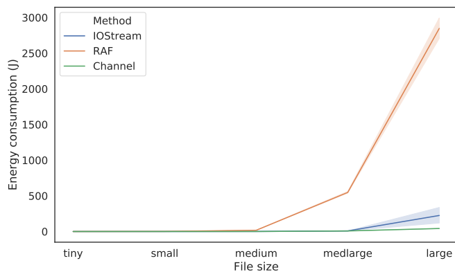
Fig. 6: Energy consumption to seek data from files of different sizes.
