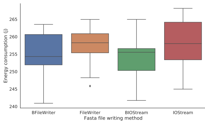
(a) Energy consumption of Fasta to generate and write 1.5 GB of nucleotide.
