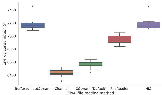
(c) Energy consumption of Zip4J to zip our large file with different read methods.
