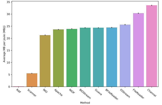
Fig. 4: The average of read data per joule for each method.
