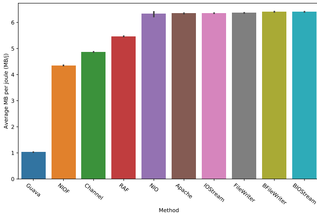
Fig. 9: The average of written data per joule for each method.
