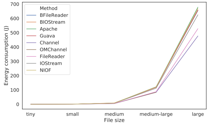
Fig. 2: Energy consumption to read files by chunks for several file sizes.
