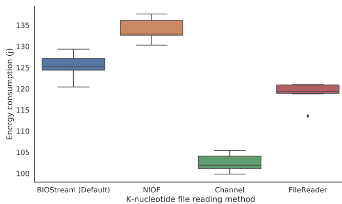
(b) Energy consumption of K-nucleotide to read the data generated by Fasta .
