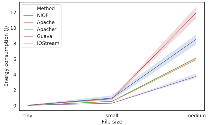
Fig. 1: Energy consumption to read the whole content of files.
