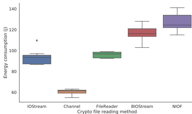
(d) Energy consumption of the Crypto library to decrypt a 3 GB file with different read methods.
