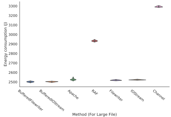
Fig. 8: Energy consumption of write methods for a large file.
