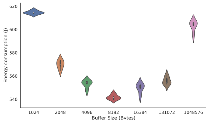
Fig. 5: Energy consumption to read files with different buffer sizes.
