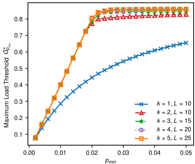
Fig. 6. Influence of parameter k : Maximum load threshold G_{p_{\min}}^* versus p_{\min} for \gamma = 0.99 , R = 0.4 and different k .
