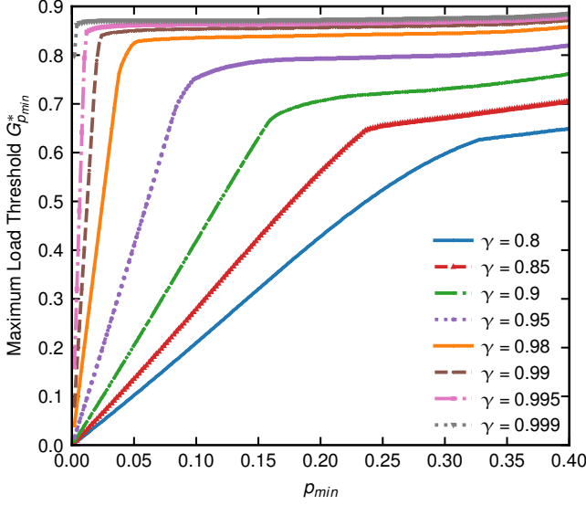
Fig. 3. Influence of parameter \gamma (1-MPR): Maximum load threshold G_{p_{\min}}^* versus p_{\min} for 3-CSA, L = 15 , R = 0.4 and different \gamma .
