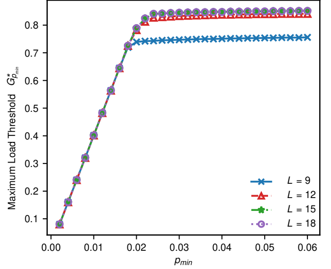
Fig. 5. Influence of parameter L : Maximum load threshold G_{p_{\min}}^* versus p_{\min} for 3-CSA, \gamma = 0.99 , R = 0.4 and different L .
