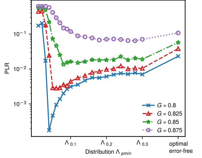
Fig. 13. PLR P_L versus \Lambda_{p_{\min}} for IRSA, \gamma = 0.99 , N = 1000 and different loads G .
