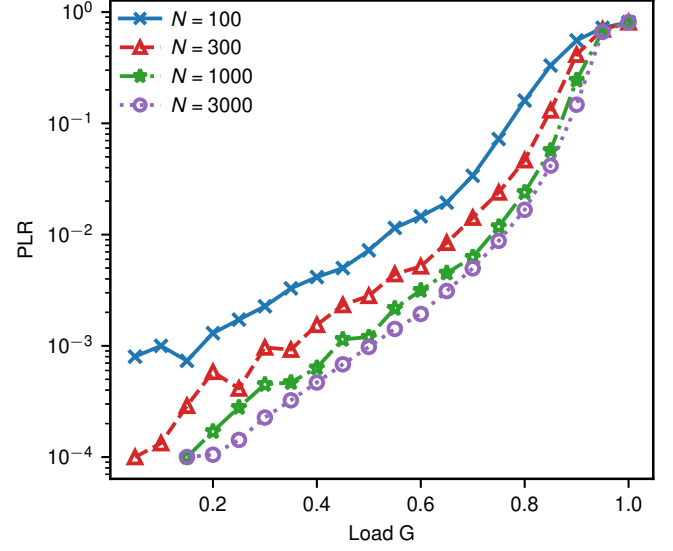
Fig. 16. Influence of N : PLR P_L versus load G for IRSA, \gamma = 0.99 , optimal error-free distribution and different N .
