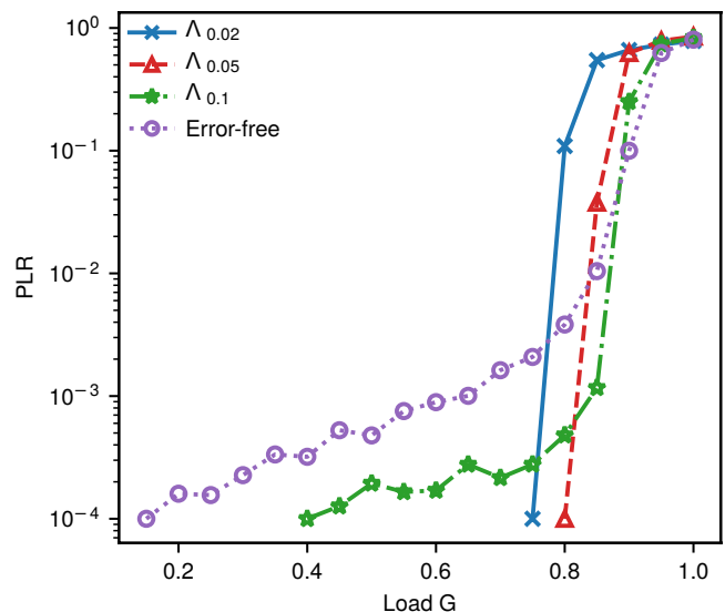
Fig. 11. PLR P_L versus load G for IRSA, \gamma = 1 , N = 1000 and different distributions \Lambda .
