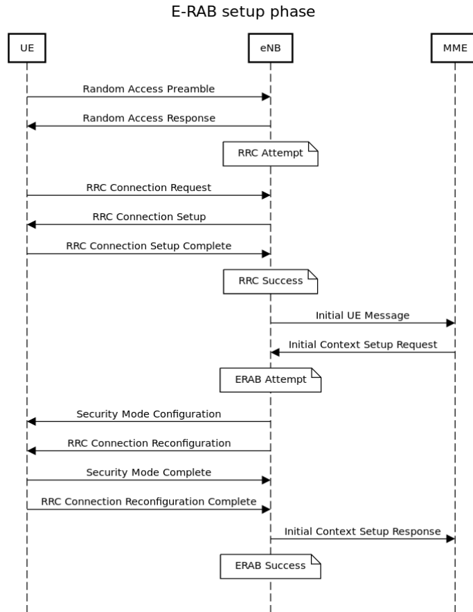
Fig. 1. Sequence diagram indicating the E-RAB setup phase.
