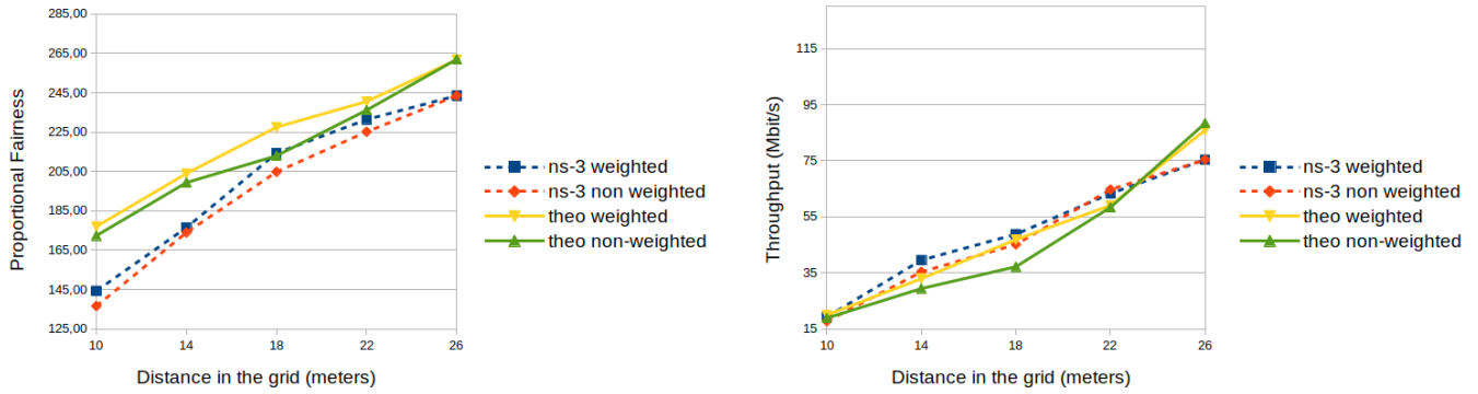
Fig. 2: Comparison of the channel allocation performance with weighted and non-weighted conflict graphs in the 5GHz band and for 20MHz channels. The distance between two APs in the grid varies. 3 channels are used.
