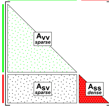
FIGURE 9: Because the coefficient matrix A of the linear system to solve (see Equation 3) is symmetric, we do not need to store the elements above the diagonal.
