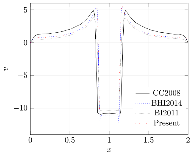
Figure 17: Comparison of the vertical velocity v on a horizontal cut through the center of the cylinder at time t = 0.1 for the sedimentation test case with data by Coquerelle and Cottet (CC2008) [46], Bergmann et al. (BHI2014) [41] and Bergmann and Iollo (BI2011) [40].
