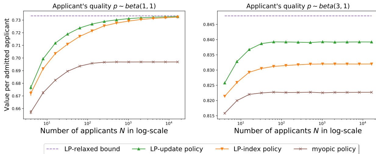
Figure 2 Performance on applicant screening problem when the decision maker knows the prior distribution of p_n (left panel) or has access to a wrong prior information (right panel).
