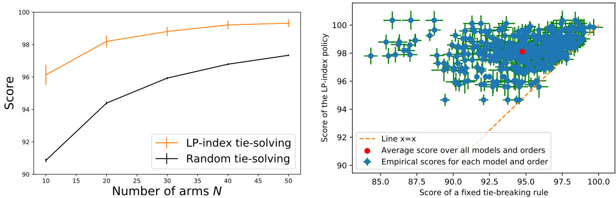
(a) Average score as a function of N (b) LP index vs arbitrary tie-solving ( N = 20 ) Figure 1 Performance of the different tie-solving among \mathcal{S}^+ and \mathcal{S}^- : LP indices, and fixed priorities. We report the normalized score (in %) as a function of the number of arms. All policies are asymptotically equivalent but the LP-index policy performs better for all finite values of N .
