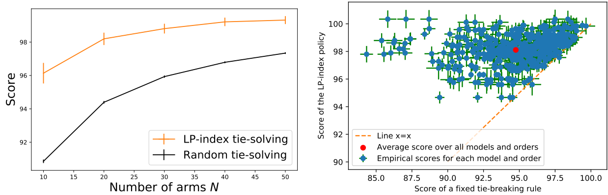
(a) Average score as a function of N (b) LP index vs arbitrary tie-solving ( N = 20 )
