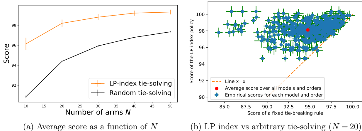
Figure 1 Performance of the different tie-solving among \mathcal{S}^+ and \mathcal{S}^- : LP indices, and fixed priorities. We report the normalized score (in %) as a function of the number of arms. All policies are asymptotically equivalent but the LP-index policy performs better for all finite values of N .
