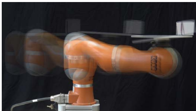
Fig. 1. A teleoperated 7-DoF robot manipulator transports an object in a nonprehensile configuration while autonomously modulating the user-specified inputs and the object orientation to prevent it from sliding and possibly falling under the action of gravity.
