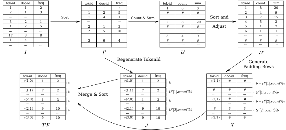
Fig. 1. Text indexing example
