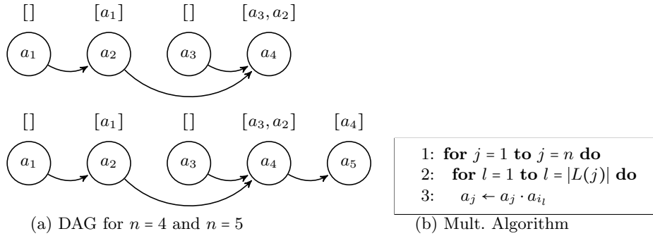
Figure 4: DAG Pre-computation and Multiplication Algorithm using DAG
