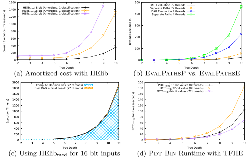
Figure 5: PDT-BIN Runtime
